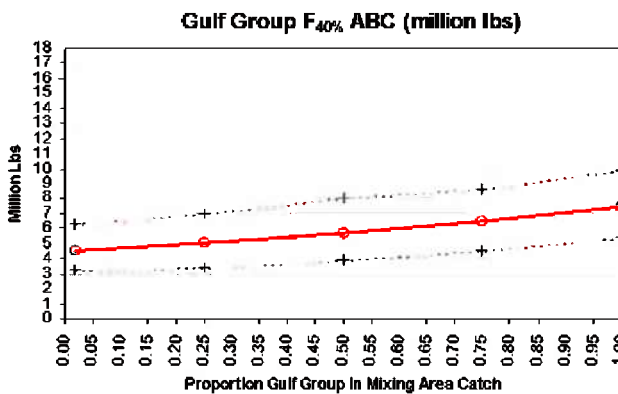
Figure 34: ABC for fishing year 2003 under either an F30%SPR (upper) or F40%SPR Fishing mortality rate for the Gulf Group (left) and Atlantic Group (right) as a function of the presumed proportion of Gulf Group fish in the annual catch taken from the mixing area. Open circles represent bootstrap medians and crosses the upper and lower 80% confidence bounds based on 500 bootstrap results. Solid and dashed lines permit interpolation should the Councils determine at a later date that alternatives to the specific scenarios modeled herein are more appropriate.
